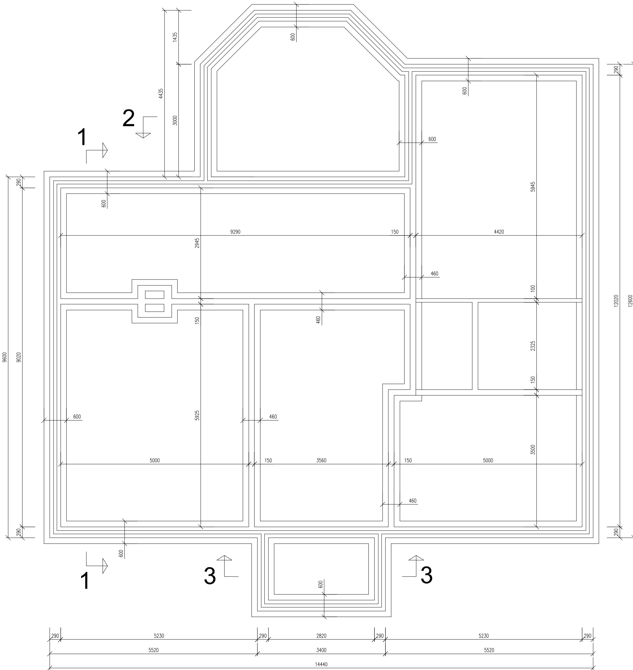
FOUNDATION PLAN
