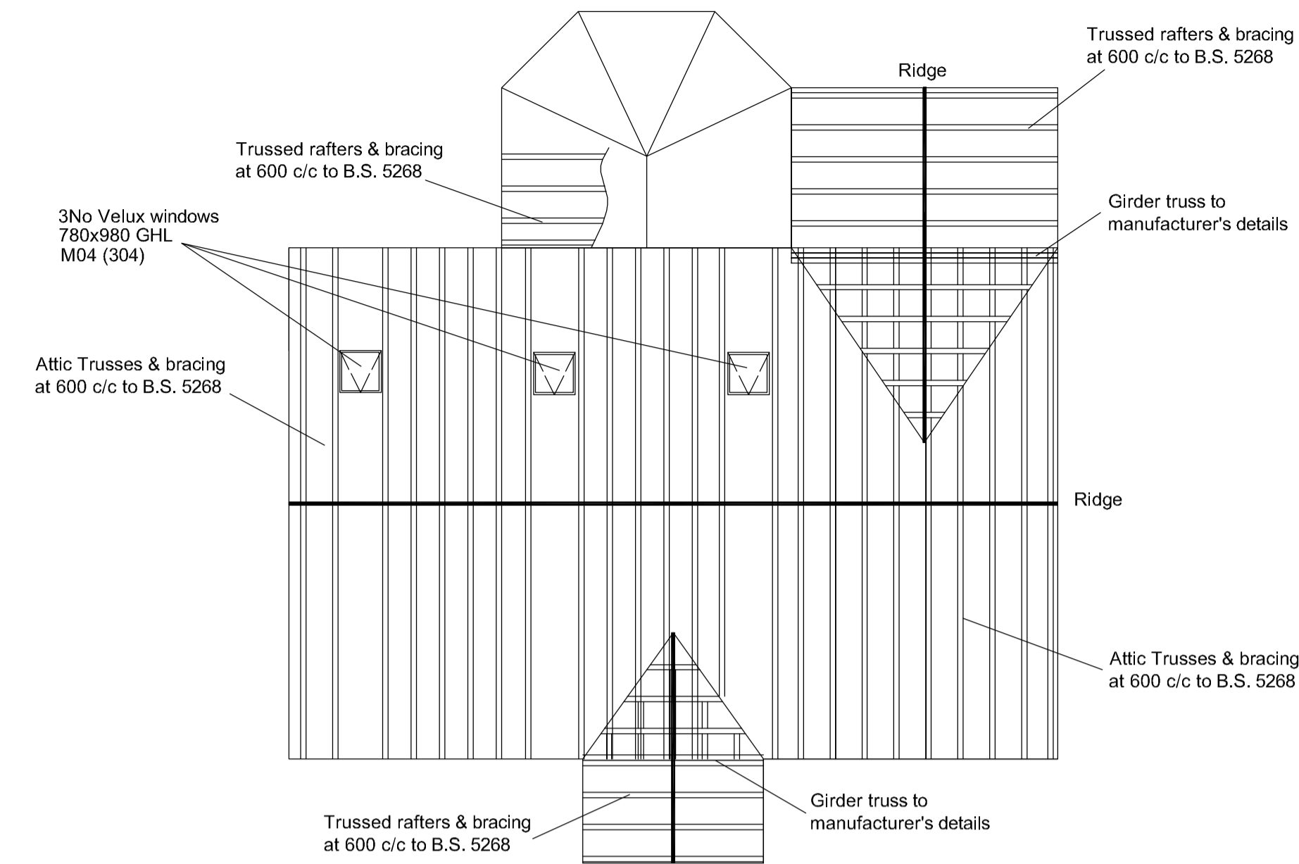
ROOF TRUSS PLAN (1:100)
